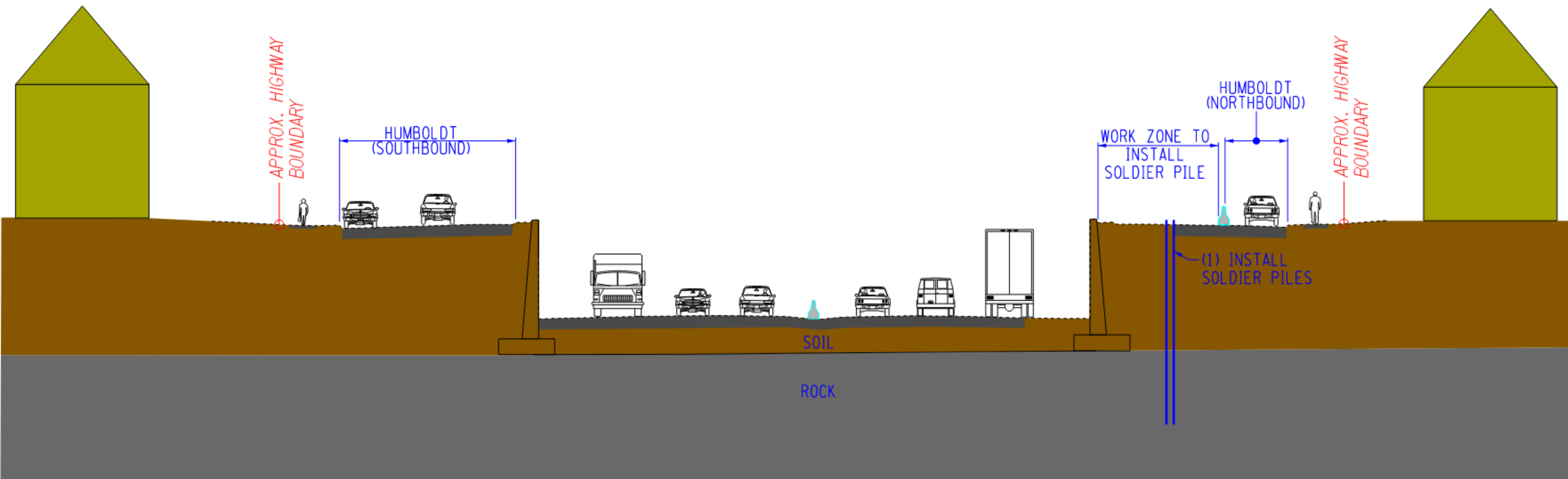
STAGE 1 - CONSTRUCT EASTBOUND TUNNEL WALLS AND ROADWAY
